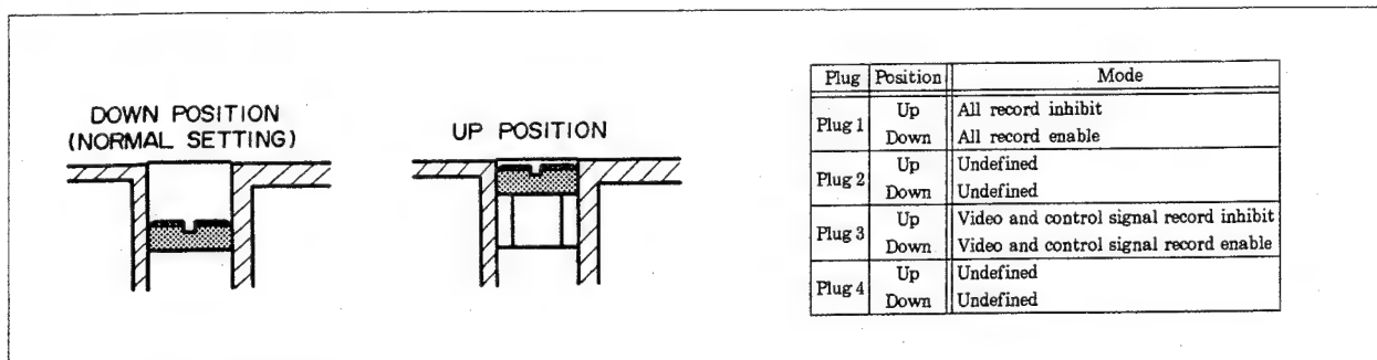
Fig. 1-2-3. User Holes/Plugs
